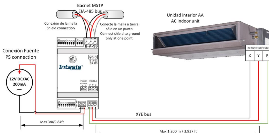
Figure 2.2 Connection diagram
